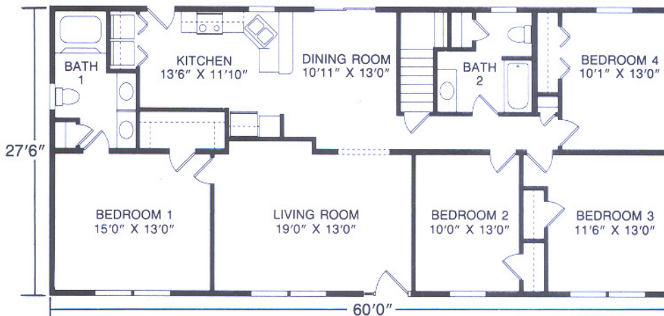
The Cameron Plan No. 361 ■ 1650 SQ. FT.
