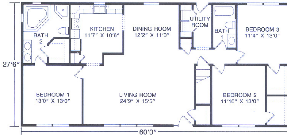
The Clemson Plan No. 360 ■ 1650 SQ. FT.
